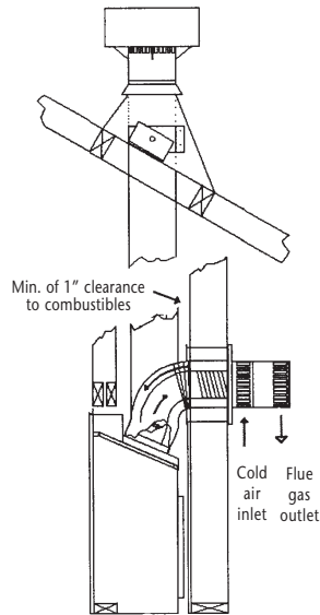
Horizontal flue option #2
